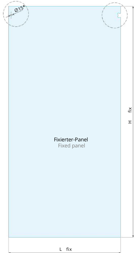
Detail C
